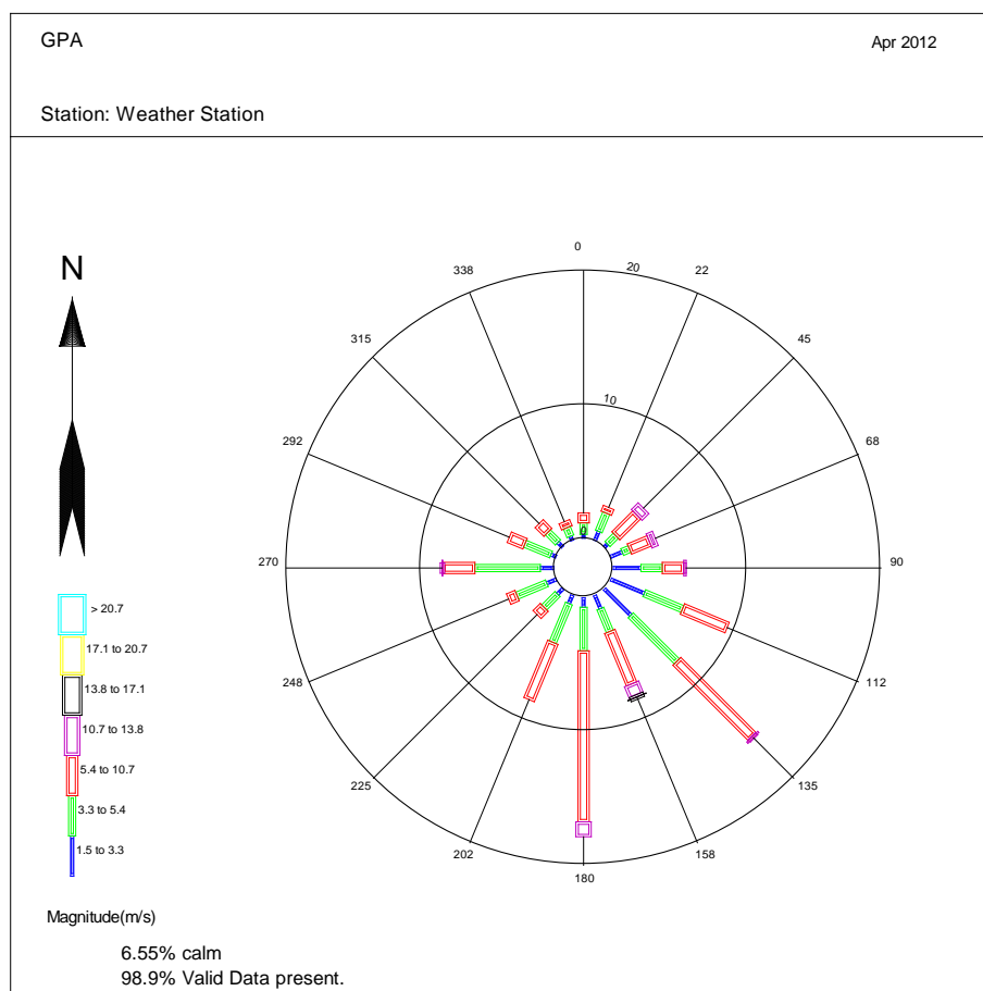
Figure 1. GPA Offshore Wind Data
